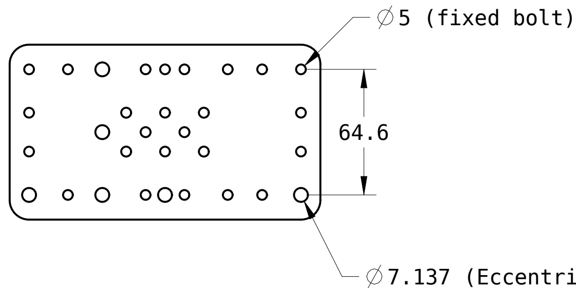
Typical wheel spacing and holes sizes
